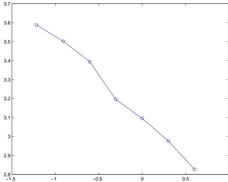
FIGURE 17.7. \|\varphi_h\|_{L_2(H^1)} corresponding to computation of the mean drag force (normalized) over a time interval [T_0, T] , as a function of the interval length |T - T_0| ( \log_{10} - \log_{10} -plot).
