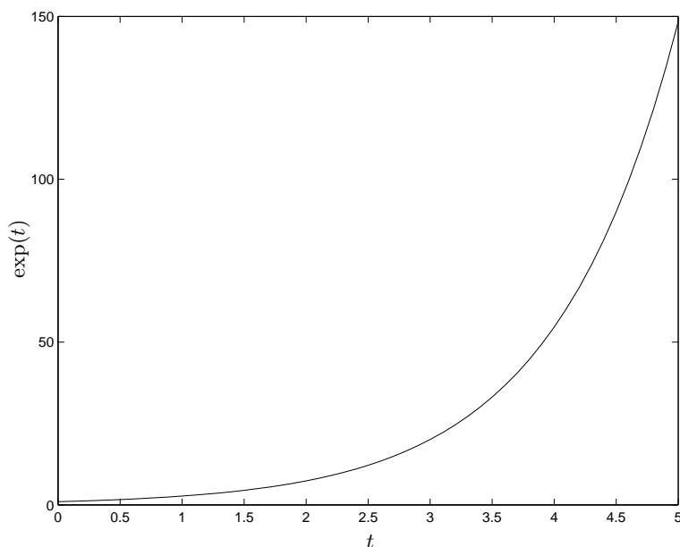
FIGURE 15.4. Graph of \exp(t) : Exponential growth.
