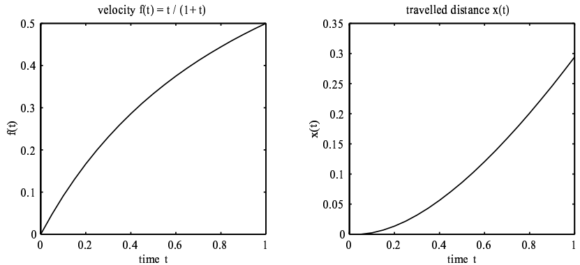
FIGURE 15.3. Travelled distance X_n approximating x(t) for f(t) = \frac{t}{1+t} with time steps k = 0.05 .
