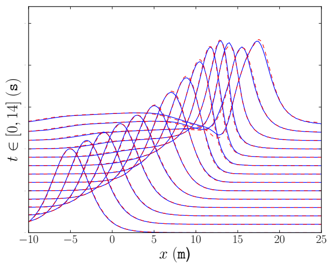
Figure 26.12: Detailed comparison of a wave passing through the trapezoidal submerged bar, simulated by DOLFWAVE using the ZTC/BEP (red dashed line) and Nwogu's BEV (blue solid line) models, for x \in [-10, 25] (m) and t \in [0, 14] (s).
