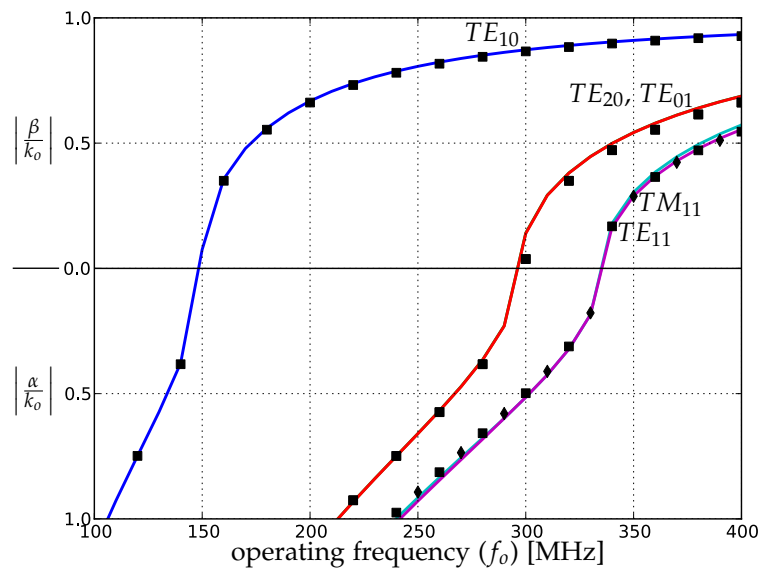
Figure 35.6: Dispersion curves for the first 5 modes of a 1\text{m} \times 0.5\text{m} hollow rectangular waveguide of Figure 35.3. Markers are used to indicate the analytical results with \blacksquare and \blacklozenge indicating TE and TM modes respectively. Note that the analytical TE_{01} and TE_{20} form a degenerate pair, as do the TE_{11} and TM_{11} modes.
