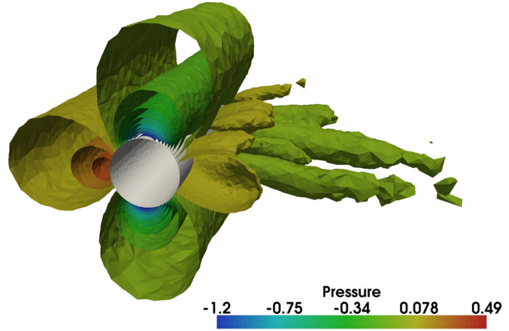
Figure 18.3: Example application of 3D turbulent incompressible flow around a cylinder with parallel adaptive computation.
