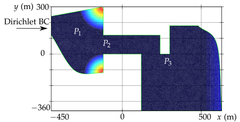
Figure 26.22: Sponge layer (viscosity \nu(x,y) ) [Max \approx 0.1 \text{ m}^2 \text{ s}^{-1} , min = 0 \text{ m}^2 \text{ s}^{-1} ].
