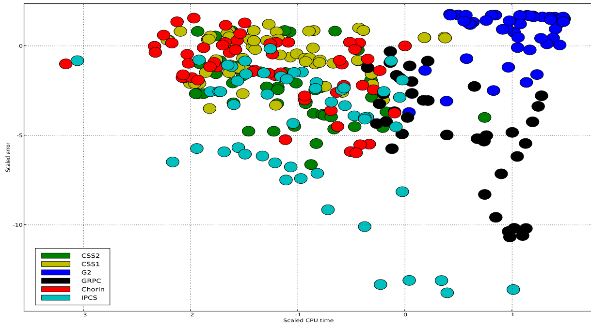
Figure 21.19: Scatter plot summarizing the results for all test problems and solvers (logarithmic scale).
