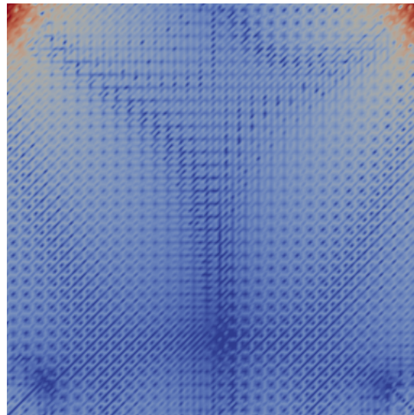
Figure 20.17: Local divergence error in lid-driven cavity using P_2 - P_1 Taylor-Hood elements. Note in particular the large error at the corners with the lid.
