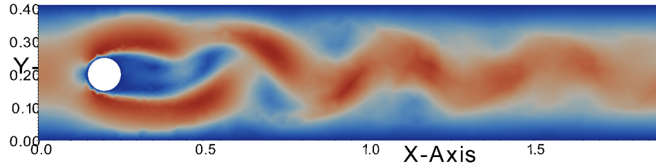
Figure 21.13: Illustration of the velocity field for the cylinder test problem at t = 5 .
