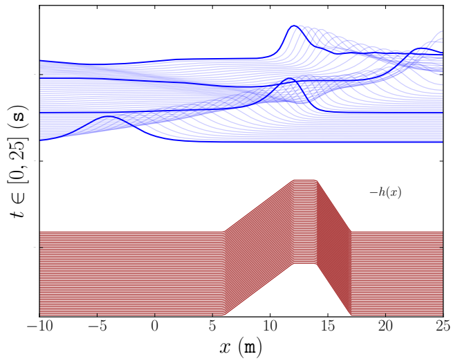
Figure 26.11: Detailed view of a wave passing through a trapezoidal submerged bar using the ZTC/BEP model implemented in DOLFWAVE
