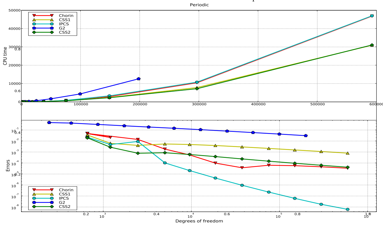
Figure 21.12: Results for the Taylor-Green vortex test problem.
