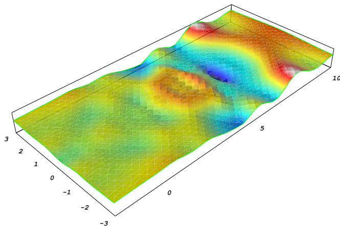
Figure 26.32: The wave surface elevation \eta (m) at the time t_3 = 6 s. [Max \approx 0.004 m, min \approx -0.006 m]
