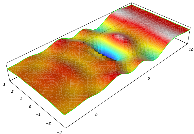
Figure 26.31: The wave surface elevation \eta (m) at the time t_2 = 4.5 s. [Max \approx 0.004 m, min \approx -0.011 m]
