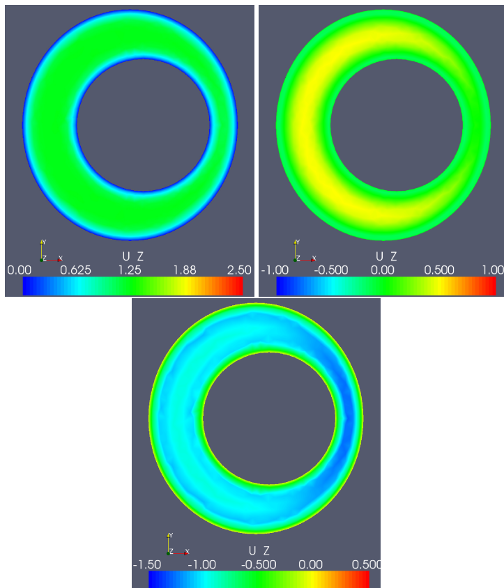
Figure 28.5: The case with circular cord and the boundary condition based on a sine function. The pictures show the velocity in z-direction as response to a sine boundary condition for the time steps t = 0.2, 0.4, 0.6 .
