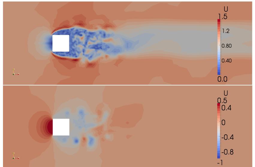
Figure 23.2: Flow around a cube: snapshots of velocity (upper) and pressure (lower) for the finest mesh.
