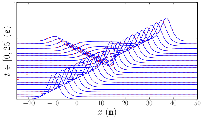
Figure 26.14: The detailed comparison of a wave passing through the triangular submerged bar with h_m = 0.1 m, \varepsilon = 0.1 , x \in [-25, 50] (m) and t \in [0, 25] (s). These solutions are provided by DOLFWAVE using the ZTC/BEP (red dashed line) and Nwogu's BEV (blue solid line) models.
