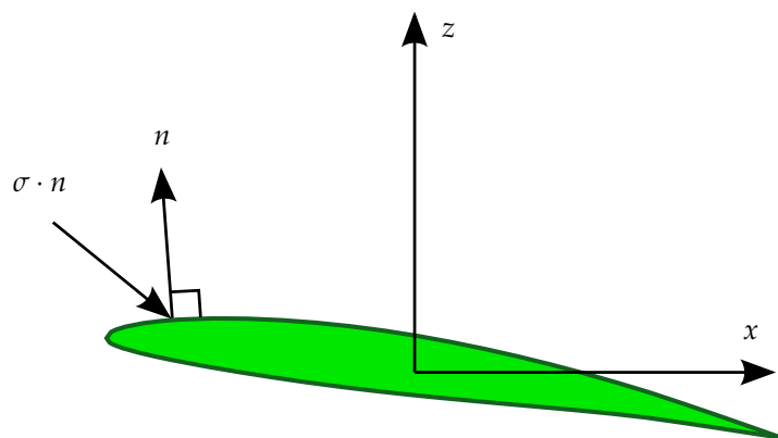
Figure 5.1: The lift and drag of an object, here a NACA 63A409 airfoil, are the integrals of the vertical and horizontal components respectively of the stress \sigma \cdot n over the surface \Gamma of the object. At each point, the product of the stress tensor \sigma and the outward unit normal vector n gives the force per unit area acting on the surface.
