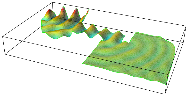
Figure 26.23: Wave surface elevation [Max \approx 0.63 \text{ m} , min \approx -0.73 \text{ m} ].
