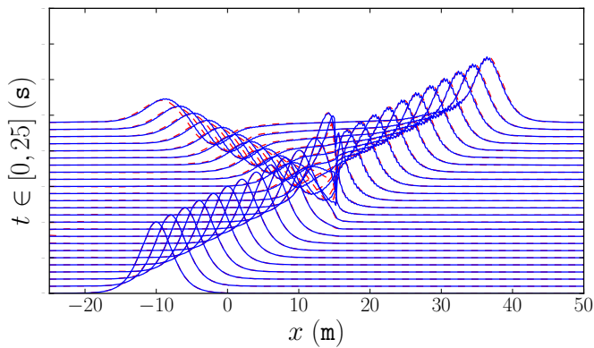
Figure 26.15: The detailed comparison of a wave passing through the triangular submerged bar with h_m = 0.04 m, \varepsilon = 0.25 , x \in [-25, 50] (m) and t \in [0, 25] (s). These solutions are provided by DOLFWAVE using the ZTC/BEP (red dashed line) and Nwogu's BEV (blue solid line) models. Small amplitude and high frequency oscillations are observed in the Nwogu's BEV model solutions.
