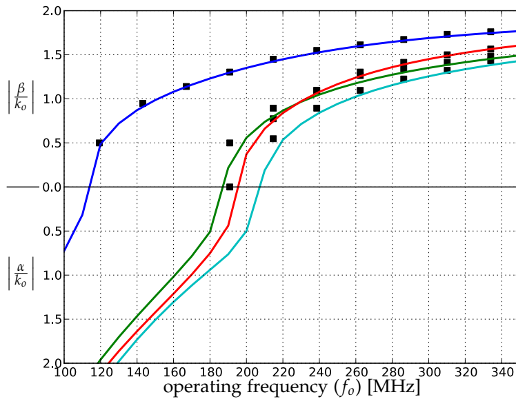
Figure 35.10: Dispersion curves for the first 4 modes of a 1\text{m} \times 0.5\text{m} half-filled rectangular waveguide as shown in Figure 35.7. Reference values for the first 4 modes from Jin [2002] are shown as ■.
