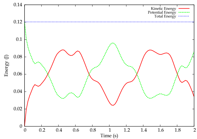
Figure 29.14: Over the course of the computation, the energy in the body is converted between potential and kinetic energy, but the total remains constant.
