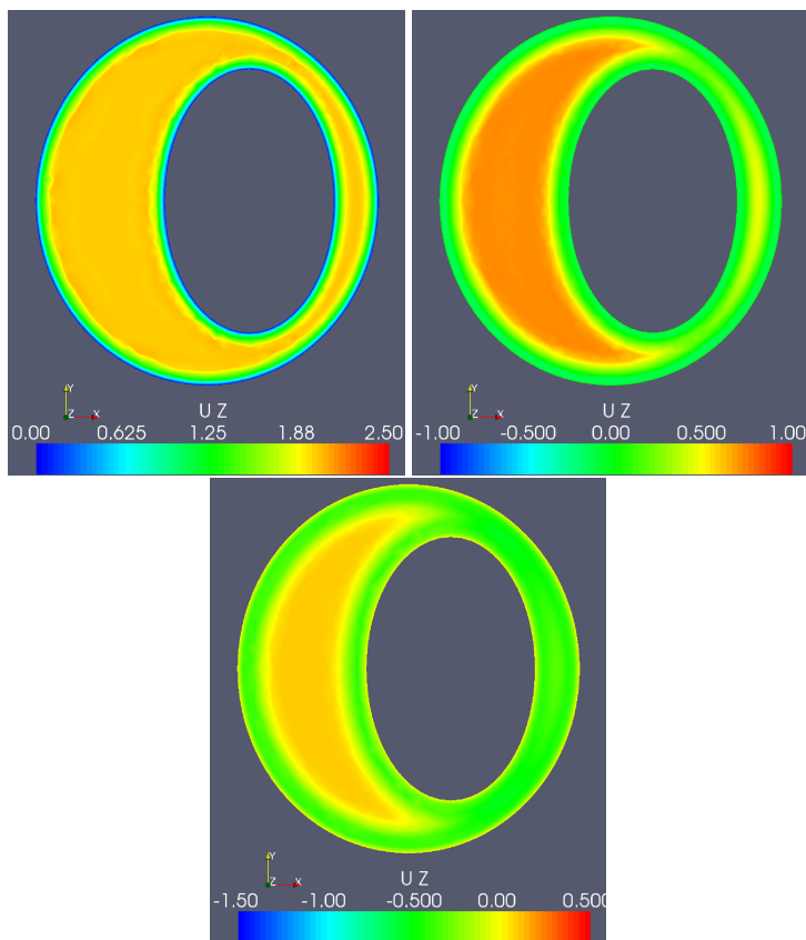
Figure 28.7: The case with a translated elliptic cord. The pictures show the velocity in z-direction for the non-symmetric pulse at the time steps t = 0.07s, 0.18s, 0.25s .
