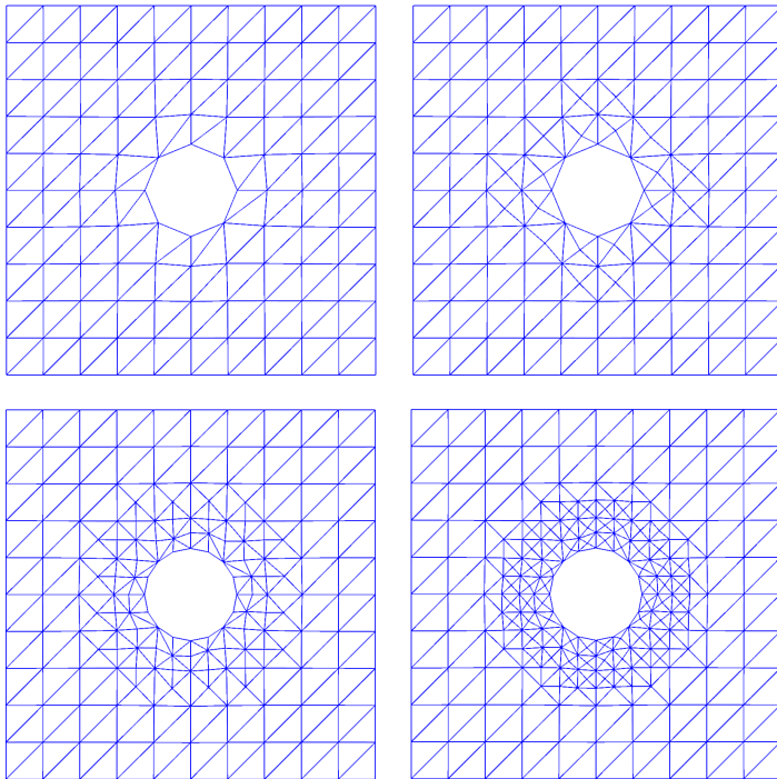
Figure 2.9: A sequence of adaptively refined meshes obtained by successive refinement of an original coarse mesh.
