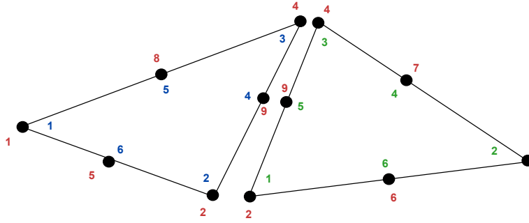
Figure 2.5: Local-to-global mapping for a simple mesh consisting of two triangles. The six local degrees of freedom of the left triangle ( T ) are mapped to the global degrees of freedom \iota_T(i) = 1, 2, 4, 9, 8, 5 for i = 1, 2, \dots, 6 , and the six local degrees of freedom of the right triangle ( T' ) are mapped to \iota_{T'}(i) = 2, 3, 4, 7, 9, 6 for i = 1, 2, \dots, 6 .
