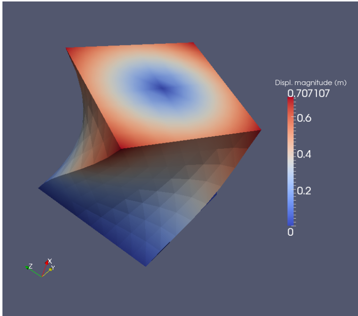
Figure 29.8: A hyperelastic cube twisted by 60 degrees.
