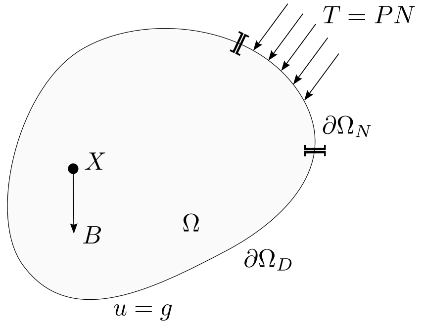
Figure 29.1: An elastic body idealized as a continuum, subjected to body forces, B , surface tractions, T , and prescribed displacement boundary conditions.
