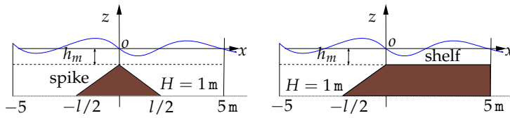
Figure 26.4: Spike and shelf geometries for the impermeable sea bottom.
