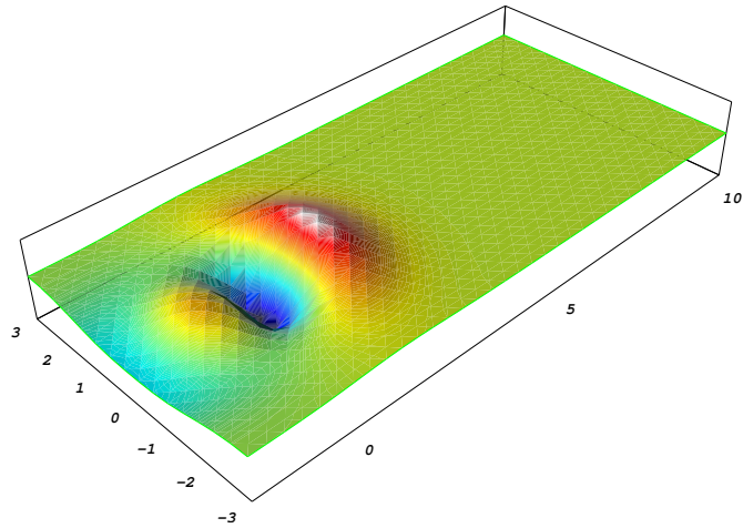
Figure 26.29: The wave surface elevation \eta (m) at the time t_0 = 1 s. [Max \approx 0.007 m, min \approx -0.010 m]
