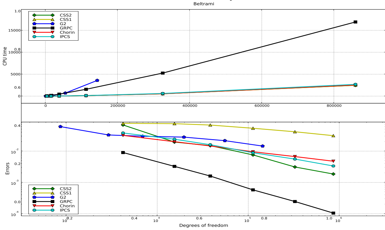
Figure 21.16: Results for the Beltrami flow test problem.
