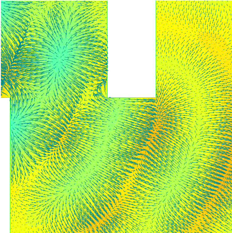
Figure 26.24: Velocity vector field at z = 0 and potential \phi_0(x, y, t_s) near P_3 . Potential values in \Omega : [Max \approx 14.2\text{m}^2\text{s}^{-1} , min \approx -12.8\text{m}^2\text{s}^{-1} ].
