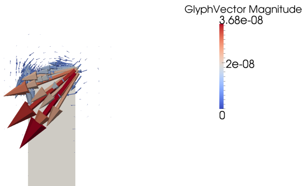
Figure 24.12: The dual mesh displacement Z_M to the channel with flap problem solved in the reference domain \Omega . The dual mesh displacement is large close to the top right corner of the structure. This is expected since the mesh in the current domain \omega(t) is significantly compressed in this region.
