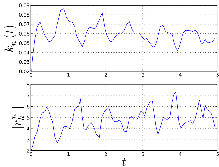
Figure 24.14: The time step k_n and the algebraic residual r_k^n as a function of time. As seen in the picture, the solution has a large variation in terms of the magnitude of the residual r_k^n .
