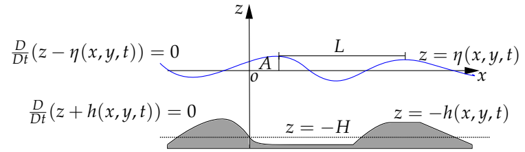
Figure 26.2: Cross-section of the water wave domain.
