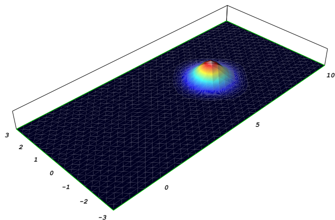
Figure 26.28: The impermeable bottom -h(x,y,t) (m) at the time t_2 = 6 s. [Max = -0.405 m, min = -0.45 m]
