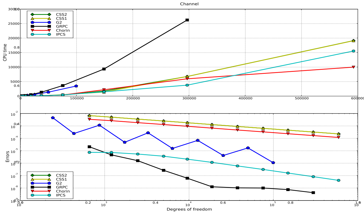
Figure 21.9: Results for the pressure-driven channel test problem.
