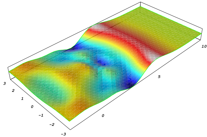
Figure 26.30: The wave surface elevation \eta (m) at the time t_1 = 3 s. [Max \approx 0.004 m, min \approx -0.006 m]
