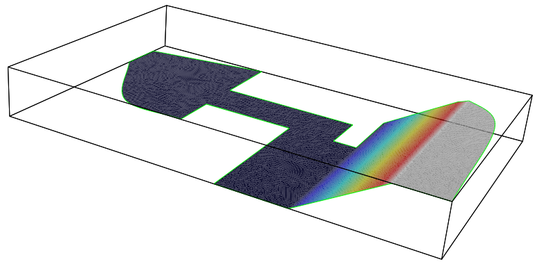
Figure 26.21: Impermeable bottom [Max = -5.316 m, min = -13.716 m].
