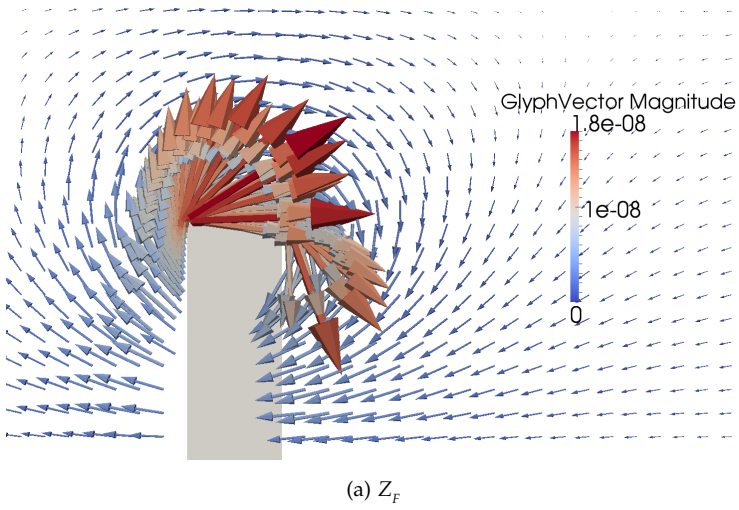
Figure 24.11: The dual fluid velocity solution Z_F and the dual structure solution Z_S at the “final time” t = 0 in the reference domain \Omega . Since the only driving force of the fully coupled dual problem is the goal functional (24.30), the dual fluid Z_F is concentrated around the top left corner of the structure where the structure displacement is large. The dual structure displacement Z_S illustrates the choice of goal functional in (24.30).
