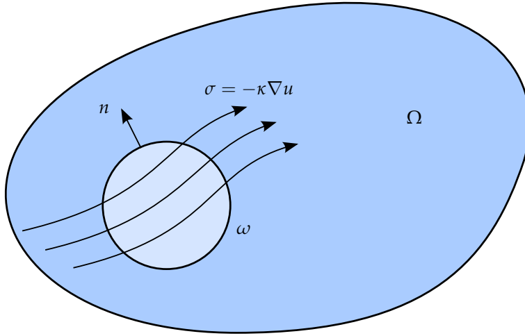
Figure 2.1: Poisson's equation is a simple consequence of balance of energy in an arbitrary test volume \omega \subset \Omega .
