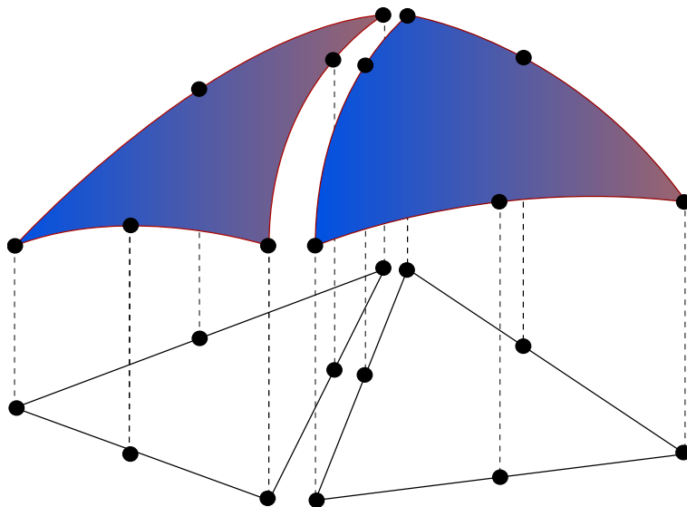
Figure 2.6: Patching together a pair of quadratic local function spaces on a pair of cells (T, T') to form a global continuous piecewise quadratic function space on \Omega = T \cup T' .
