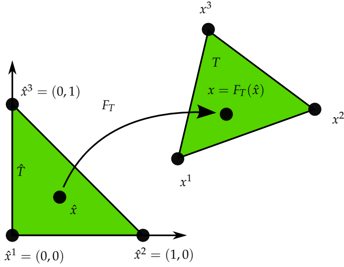
Figure 8.1: The (affine) map F_T from a reference cell \hat{T} to a cell T \in \mathcal{T}_h .
