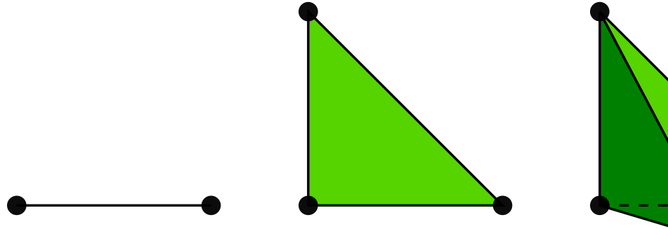
Figure 3.2: The linear Lagrange interval, triangle and tetrahedron.
