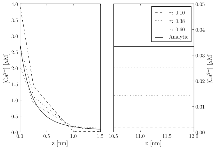
Figure 34.6: The figure shows the concentration traces of the numerical solutions from Mesh 3 (see legend of Figure 34.3), for three different \tau , together with the analytical solution. The traces in the two panels were picked from the same lines for Figure 34.5. Again, we see from both panels that the solution with \tau = 0.10 give the poorest solution. The solution with \tau = 0.38 was the solution with smallest global error for this mesh (see Fig 34.3), and this is reflected in the good fit seen in the left panel, especially at z = 0 nm. The solution with \tau = 0.60 undershoots the analytical solution at z = 0 with \simeq 0.7 \mu\text{M} . From the right panel, we see that all numerical solutions undershoot at z = 15 nm, and the trace with \tau = 0.60 here also comes closest to the analytical solution.
