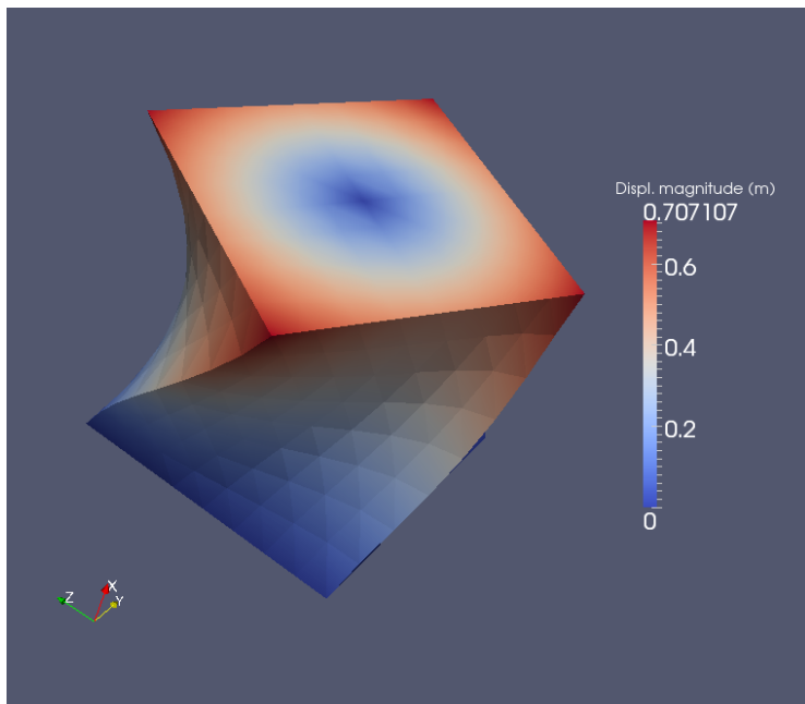
Figure 30.8: A hyperelastic cube twisted by 60 degrees.
