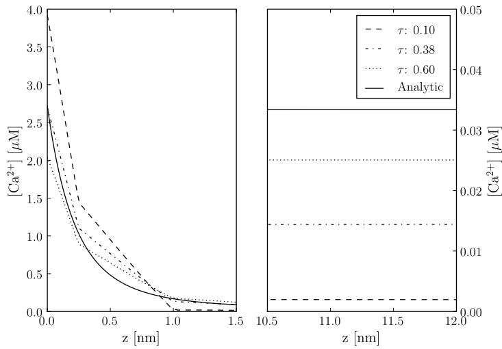
Figure 35.6: The figure shows the concentration traces of the numerical solutions from Mesh 3 (see legend of Figure ??), for three different \tau , together with the analytical solution. The traces in the two panels were picked from the same lines for Figure ?. Again, we see from both panels that the solution with \tau = 0.10 give the poorest solution. The solution with \tau = 0.38 was the solution with smallest global error for this mesh (see Fig ??), and this is reflected in the good fit seen in the left panel, especially at z = 0 nm. The solution with \tau = 0.60 undershoots the analytical solution at z = 0 with \simeq 0.7 \mu\text{M} . From the right panel, we see that all numerical solutions undershoot at z = 15 nm, and the trace with \tau = 0.60 here also comes closest to the analytical solution.
