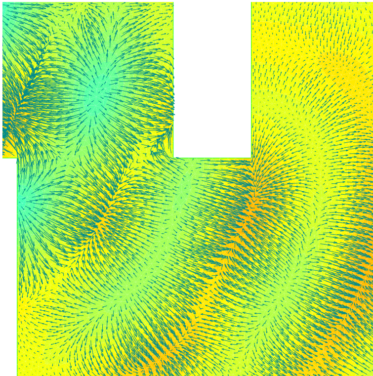
Figure 27.24: Velocity vector field at z = 0 and potential \phi_0(x, y, t_s) near P_3 . Potential values in \Omega : [Max \approx 14.2 \text{ m}^2 \text{ s}^{-1} , min \approx -12.8 \text{ m}^2 \text{ s}^{-1} ].
