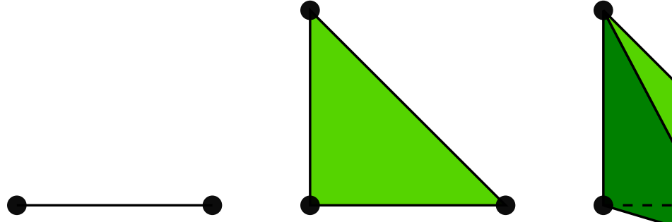
Figure 4.2: The linear Lagrange interval, triangle and tetrahedron.
