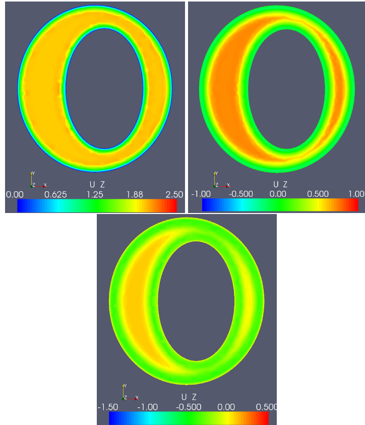
Figure 29.6: The case with an elliptic cord and the boundary condition based on the pressure pulse in the heart. The pictures show the velocity in z-direction for the non-symmetric pulse at the time steps t = 0.07s, 0.18s, 0.25s .
