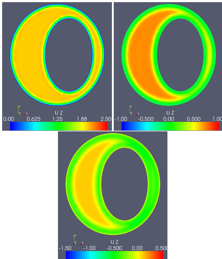
Figure 29.7: The case with a translated elliptic cord. The pictures show the velocity in z-direction for the non-symmetric pulse at the time steps t = 0.07s, 0.18s, 0.25s .
