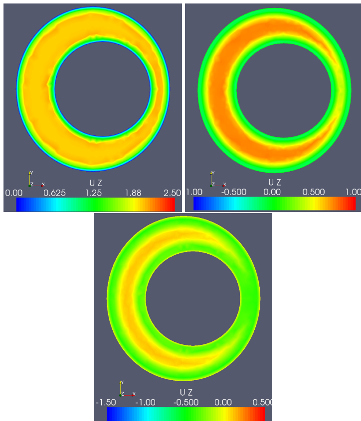
Figure 29.4: The case with a circular cord and the boundary condition based on the pressure pulse in the heart [Smith et al., 2006]. The pictures show the velocity in z-direction for the non-symmetric pulse at the time steps t = 0.07s, 0.18s, 0.25s . Notice that we use different color scales for the different time steps. The same color scales will be used in all subsequent figures.
