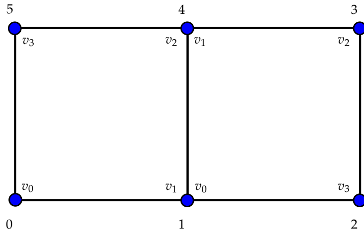
Figure 17.5: The local numbering of vertices of a non-simplicial mesh is arbitrary, as long as each cell is topologically isomorphic to the reference cell by matching each vertex to the corresponding vertex of the reference cell.
