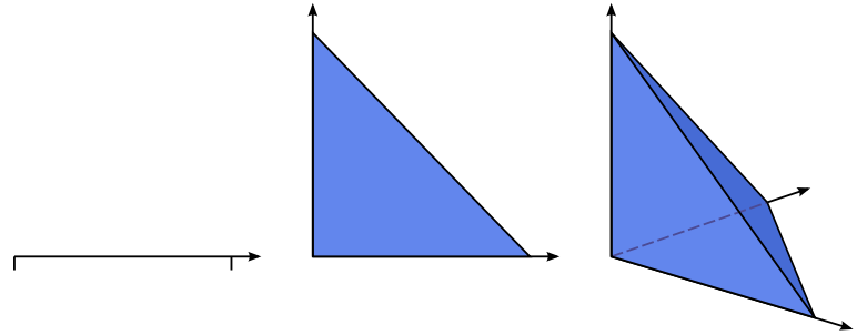
Figure 3.2: Examples of finite element cells in one, two and three space dimensions.
