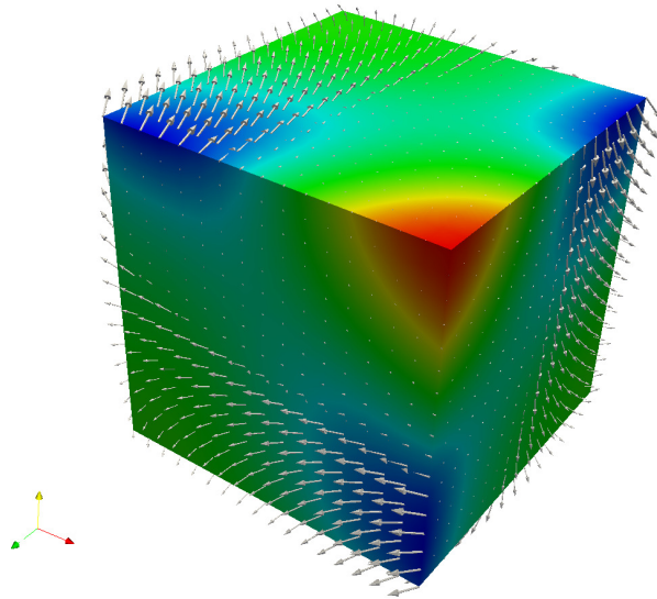
Figure 22.15: Solution of the Beltrami flow test problem.
