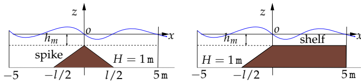
Figure 27.4: Spike and shelf geometries for the impermeable sea bottom.
