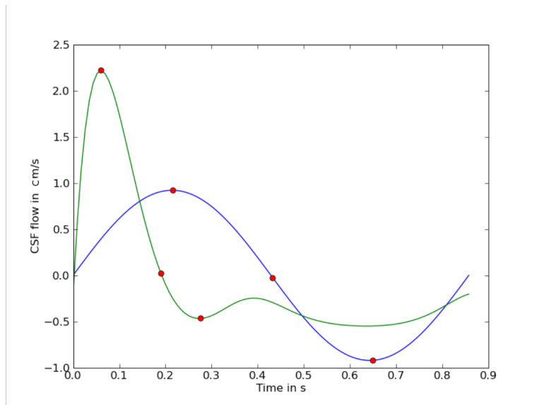
Figure 29.2: Two different CSF flow pulses. The blue line is a sine pulse, whereas the green is derived from the pressure pulse in a heart chamber.
