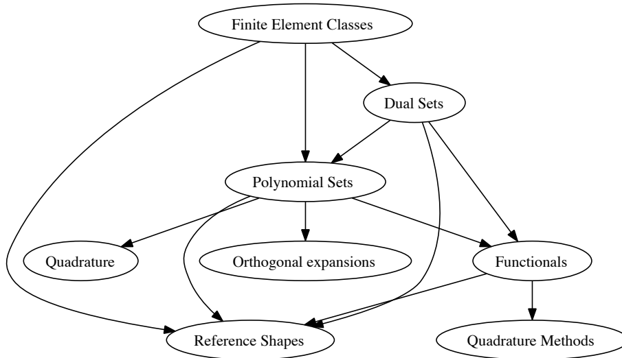
Figure 14.3: General relationship between the kinds of classes in FIAT.
