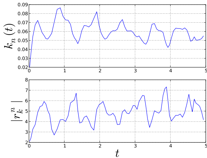
Figure 25.14: The time step k_n and the algebraic residual r_k^n as a function of time. As seen in the picture, the solution has a large variation in terms of the magnitude of the residual r_k^n .
