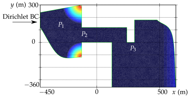
Figure 27.22: Sponge layer (viscosity \nu(x, y) ) [Max \approx 0.1\text{m}^2\text{s}^{-1} , min = 0\text{m}^2\text{s}^{-1} ].
