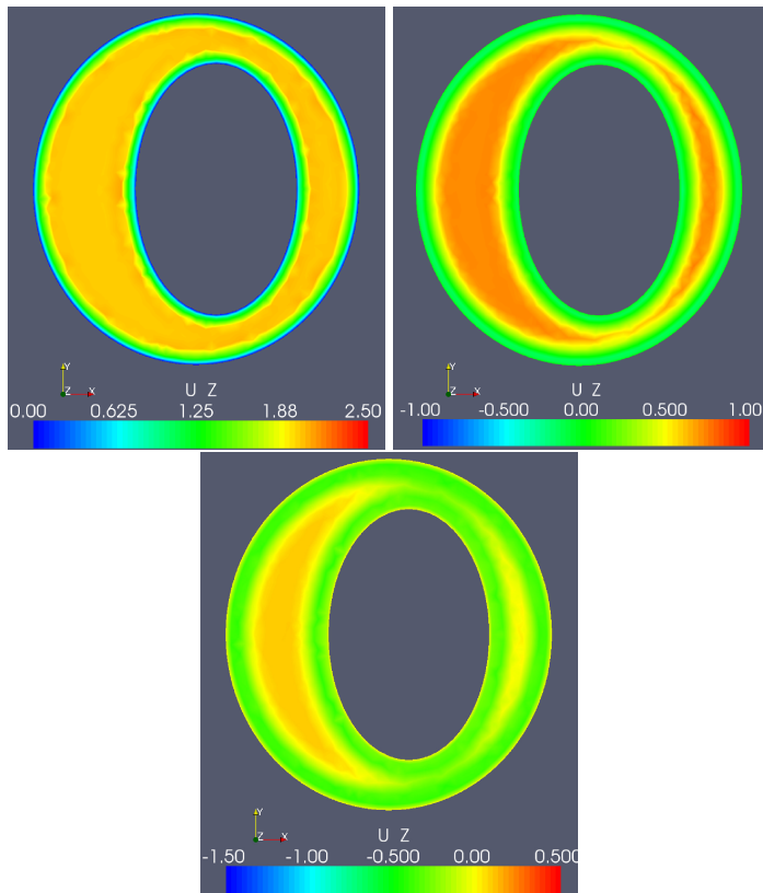
Figure 29.6: The case with an elliptic cord and the boundary condition based on the pressure pulse in the heart. The pictures show the velocity in z -direction for the non-symmetric pulse at the time steps t = 0.07s, 0.18s, 0.25s .
