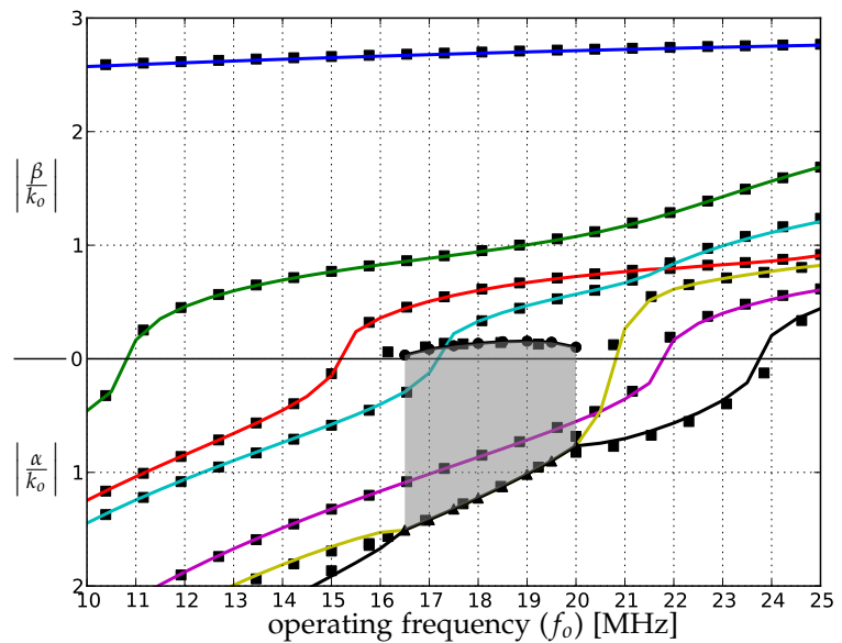
Figure 36.12: Dispersion curves for the first 7 even modes of shielded microstrip line of Figure 36.11 using a magnetic wall to enforce symmetry. Reference values from Pelosi et al. [1998] are shown as \blacksquare . The presence of complex mode pairs are indicated by \blacktriangle and \bullet and highlighted in grey.
