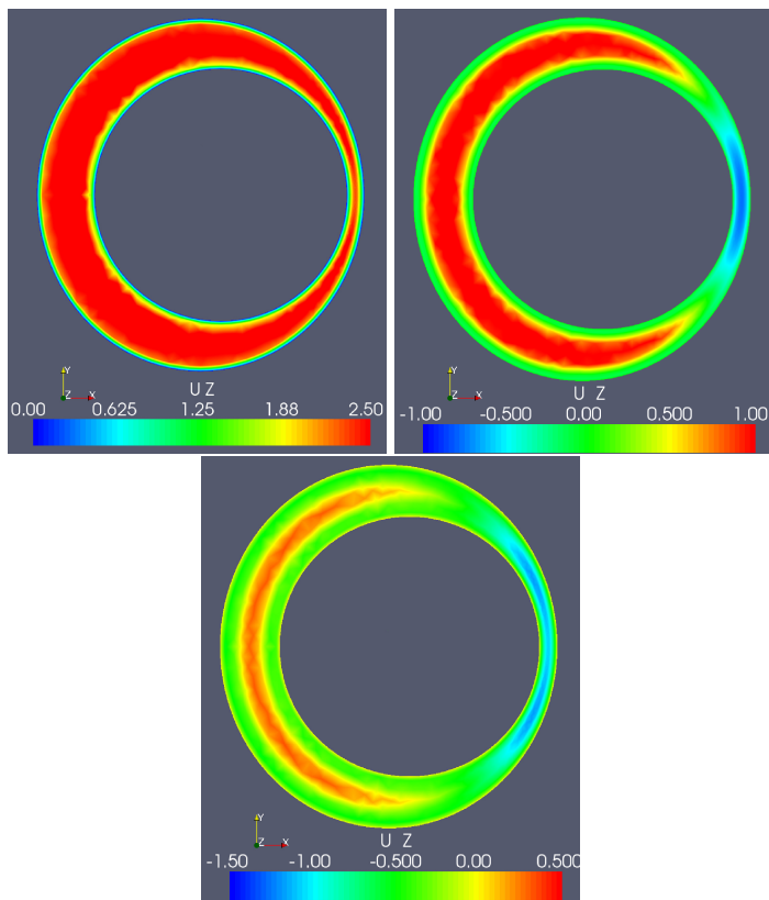
Figure 29.8: The case with an enlarged cord diameter and the boundary conditions based on the pressure pulse. The pictures show the velocity in z -direction for the non-symmetric pulse at the time steps t = 0.07s, 0.18s, 0.25s .
