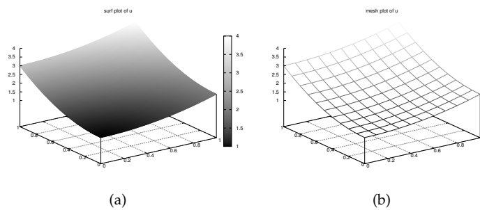
Figure 2.6: Examples on plots created by transforming the finite element field to a field on a uniform, structured 2D grid: (a) a surface plot of the solution; (b) lifted mesh plot of the solution.
