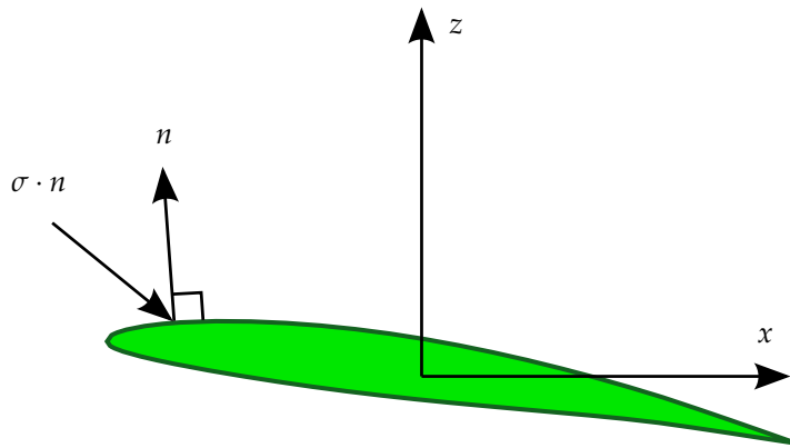
Figure 6.1: The lift and drag of an object, here a NACA 63A409 airfoil, are the integrals of the vertical and horizontal components respectively of the stress \sigma \cdot n over the surface \Gamma of the object. At each point, the product of the stress tensor \sigma and the outward unit normal vector n gives the force per unit area acting on the surface.
