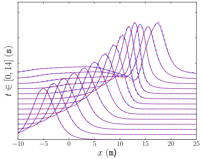
Figure 27.12: Detailed comparison of a wave passing through the trapezoidal submerged bar, simulated by DOLFWAVE using the ZTC/BEP (red dashed line) and Nwogu's BEV (blue solid line) models, for x \in [-10, 25] (m) and t \in [0, 14] (s).
