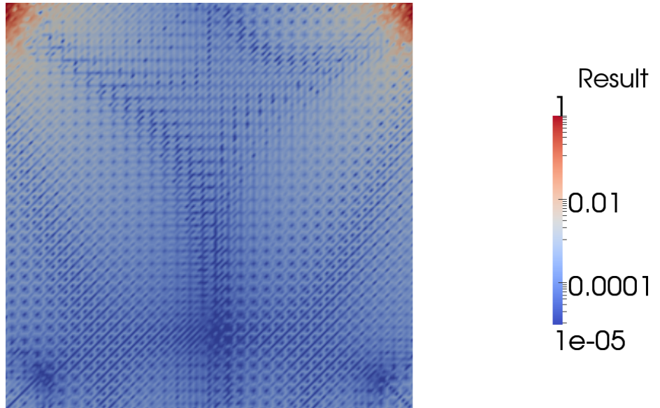
Figure 21.17: Local divergence error in lid-driven cavity using P_2 - P_1 Taylor-Hood elements. Note in particular the large error at the corners with the lid.
