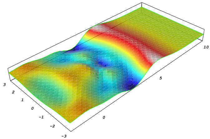
Figure 27.31: The wave surface elevation \eta (m) at the time t_2 = 4.5 s. [Max \approx 0.004 m, min \approx -0.011 m]
