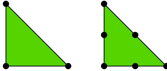
Figure 5.2: Lagrange elements of order one and two.
